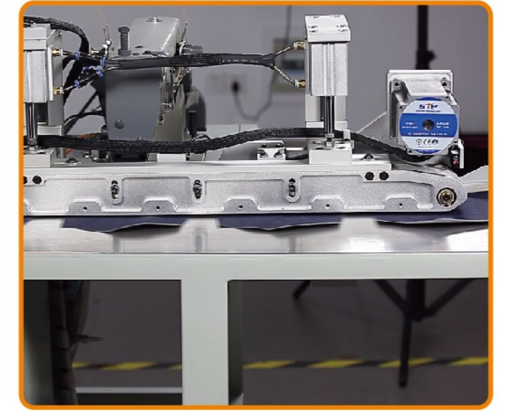
Automatic Pocket mouth curling machine
