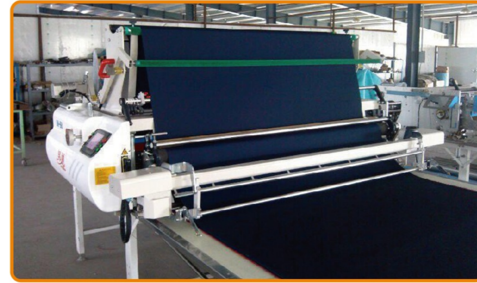
Automatic Fabric Spreading Machine
